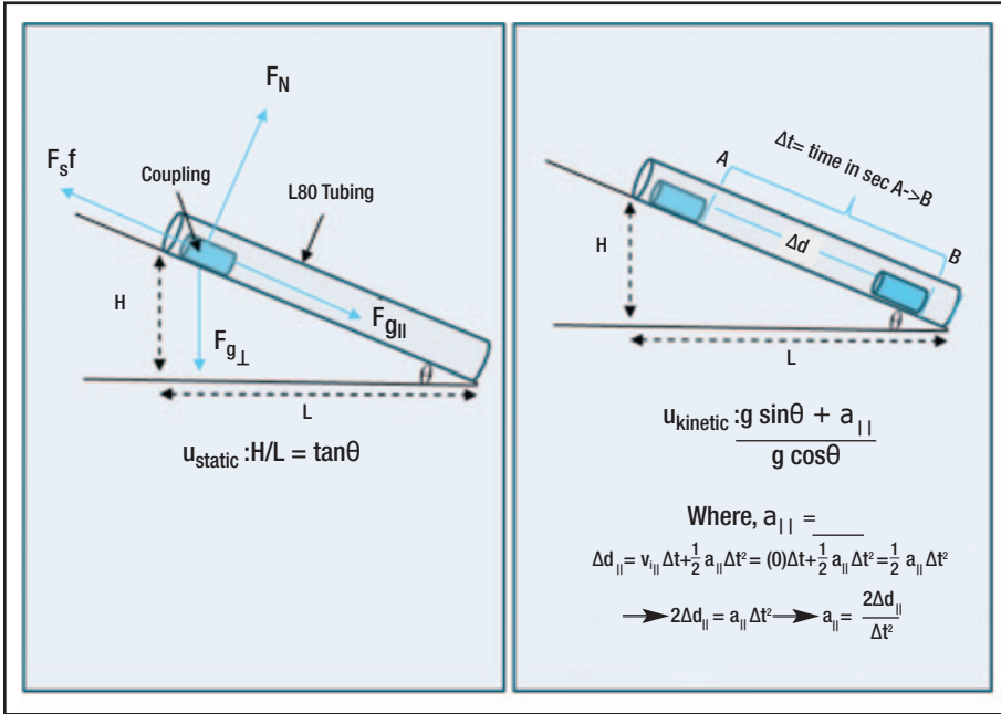
FIGURE 2 Static (left) and Kinetic (right) Coefficient of Friction
